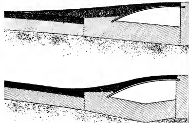
Cross Section Drawings. Corrugated Iron Part Circle for Driveways and Alleys.
